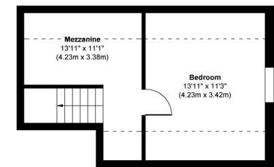
First Floor Approximate Floor Area 288 sq. ft (26.80 sq. m)
