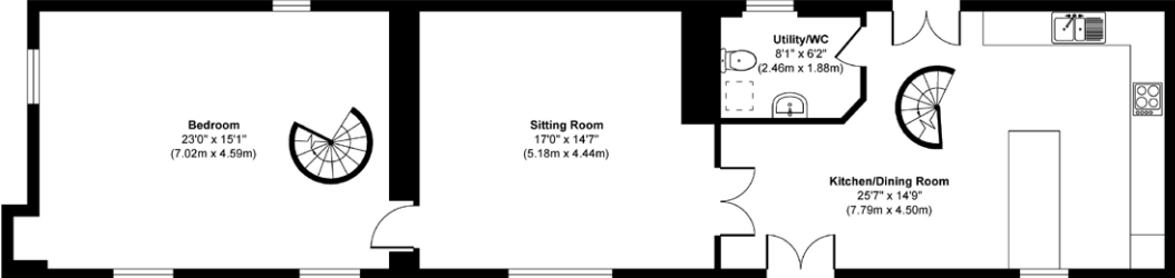
Ground Floor Approximate Floor Area 966 sq. ft (89.83 sq. m)
