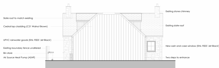
④ Proposed North Elevation 1 : 100
