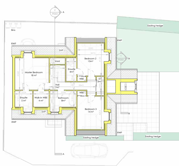
② Proposed First Floor Plan 1 : 100
