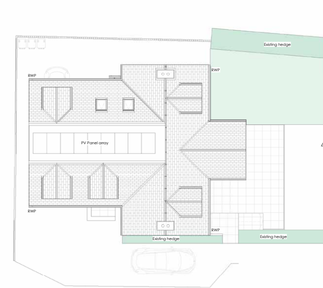
③ Proposed Roof Plan 1 : 100
