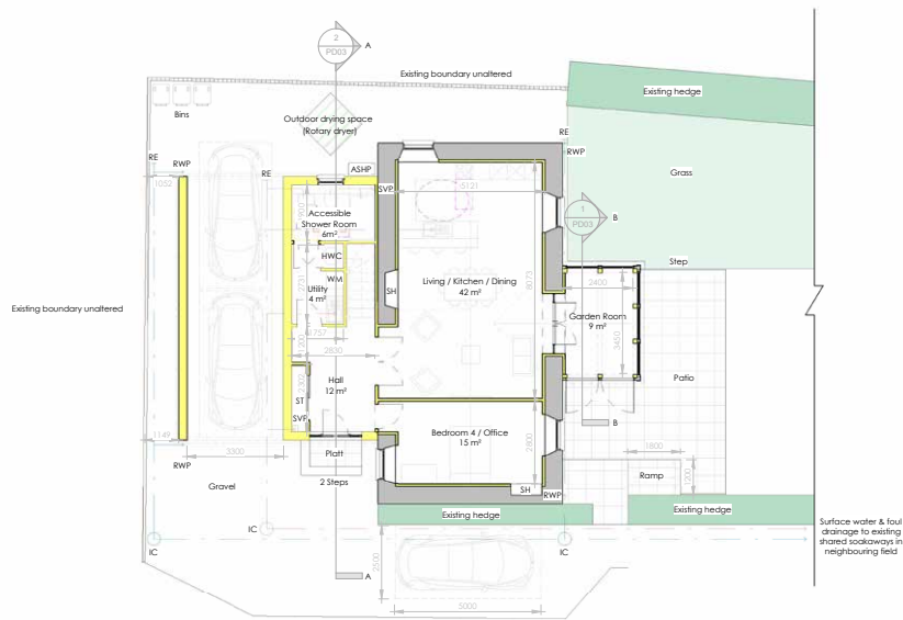
① Proposed Ground Floor Plan 1 : 100
