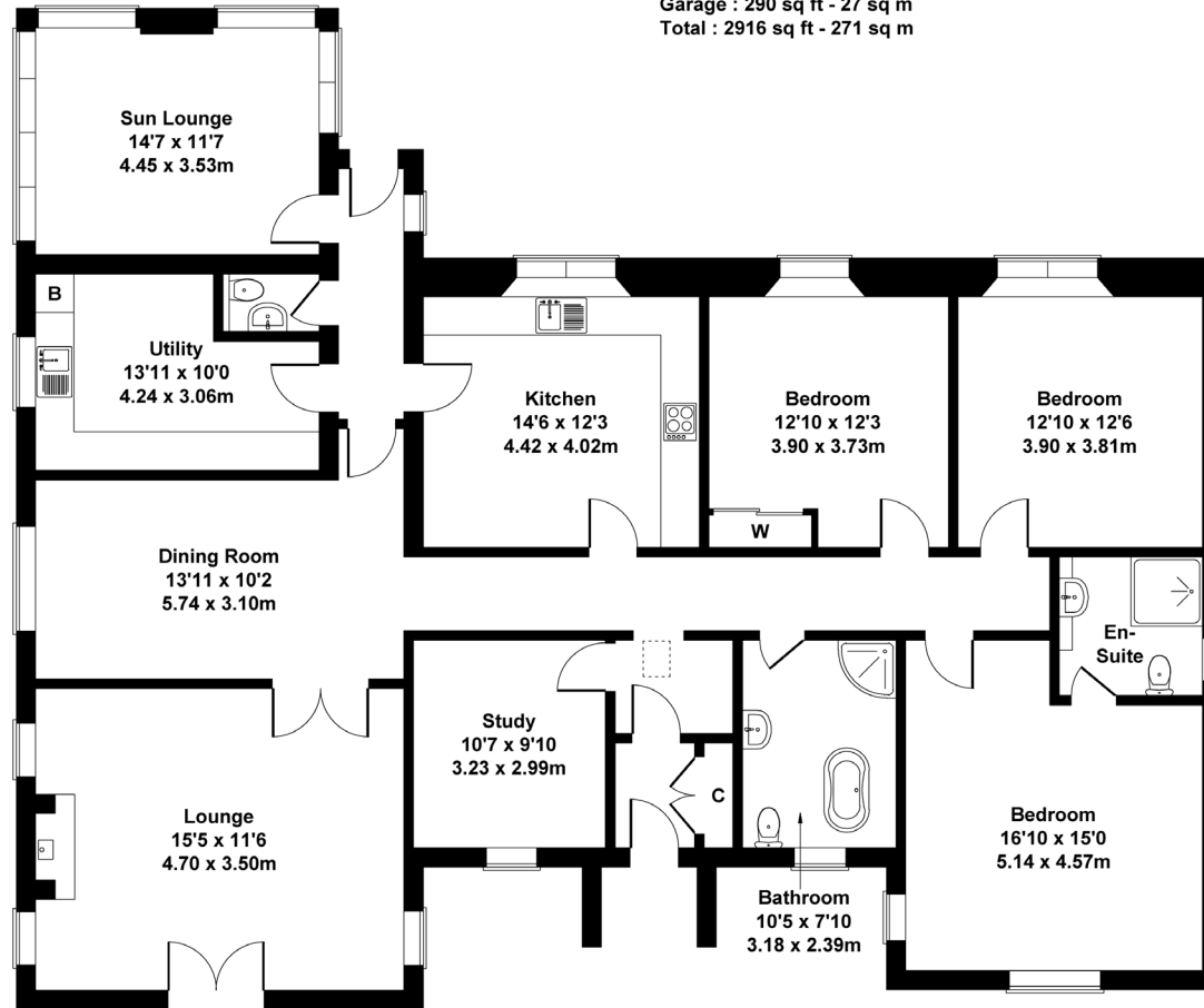
GROUND FLOOR
